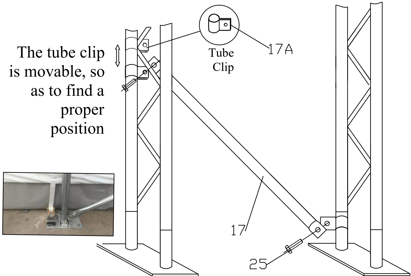
Figure 6: Wind Brace Supports(part 17)
