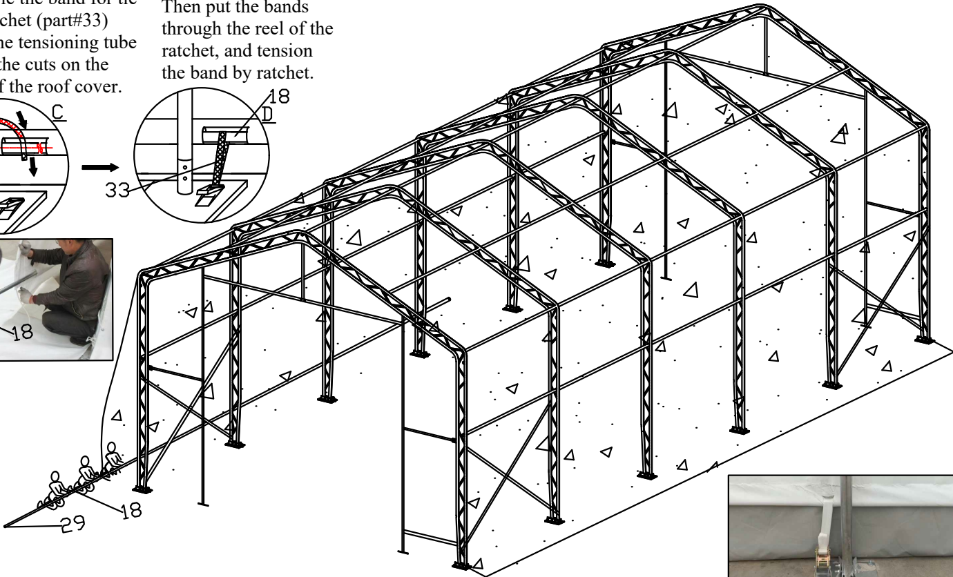
Figure 9 Fastening the Roof Cover
