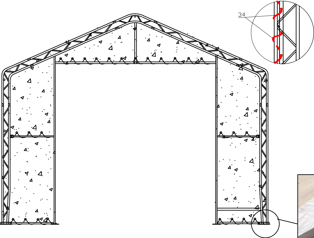
Figure 10 Installation of Front Panel Cover
