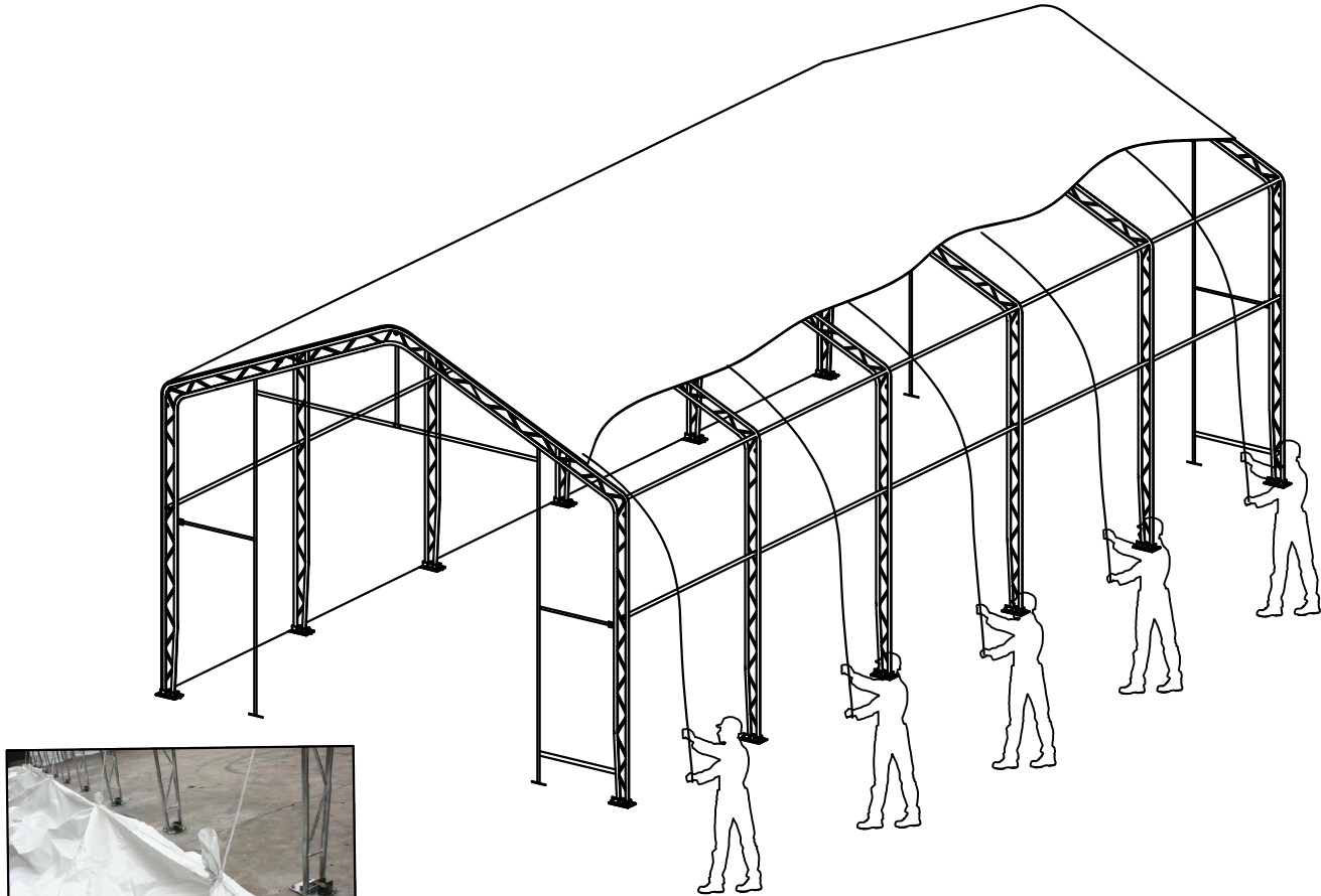
Figure 8 Pull the Roof Cover over the frame evenly
