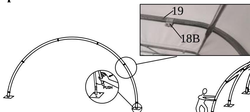
Figure 6 Attaching Arches to Base Flanges
