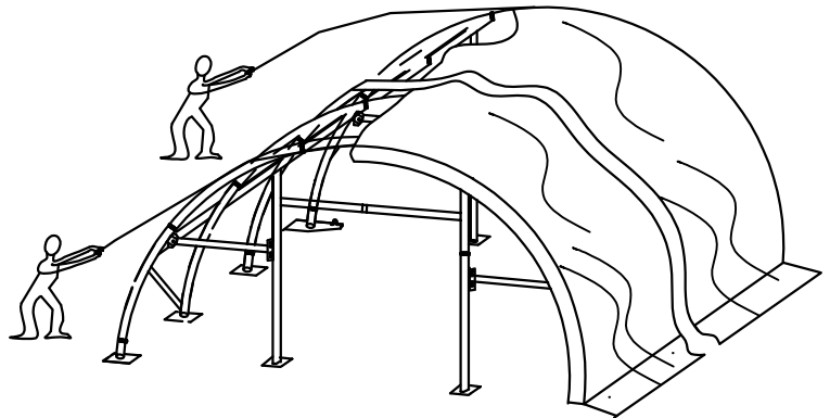
Figure8: Pull the Roof Cover over the frame evenly
