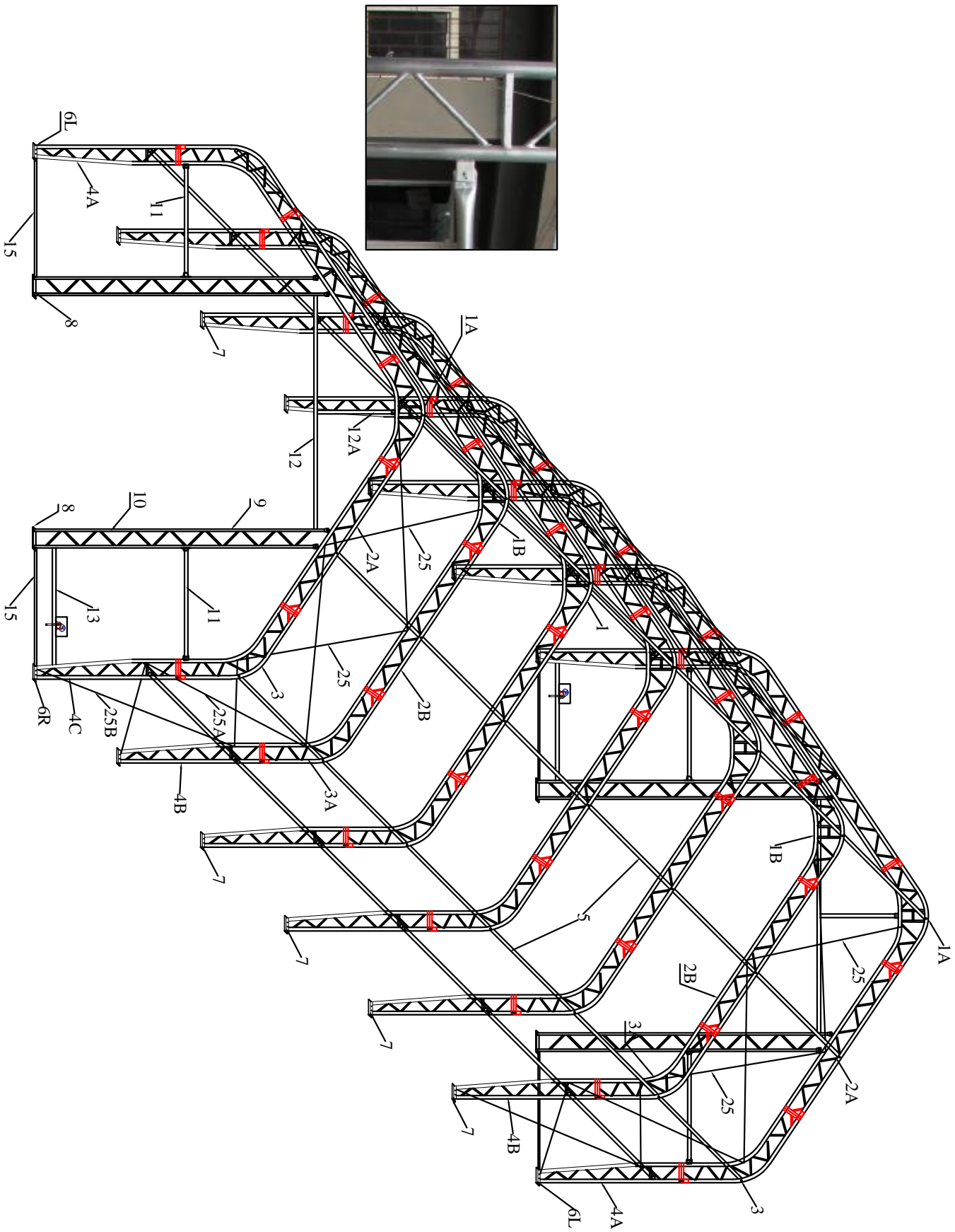
Figure 1 Sketch of Model 306022T Size: W9. 15*L18. 288*6.7M
