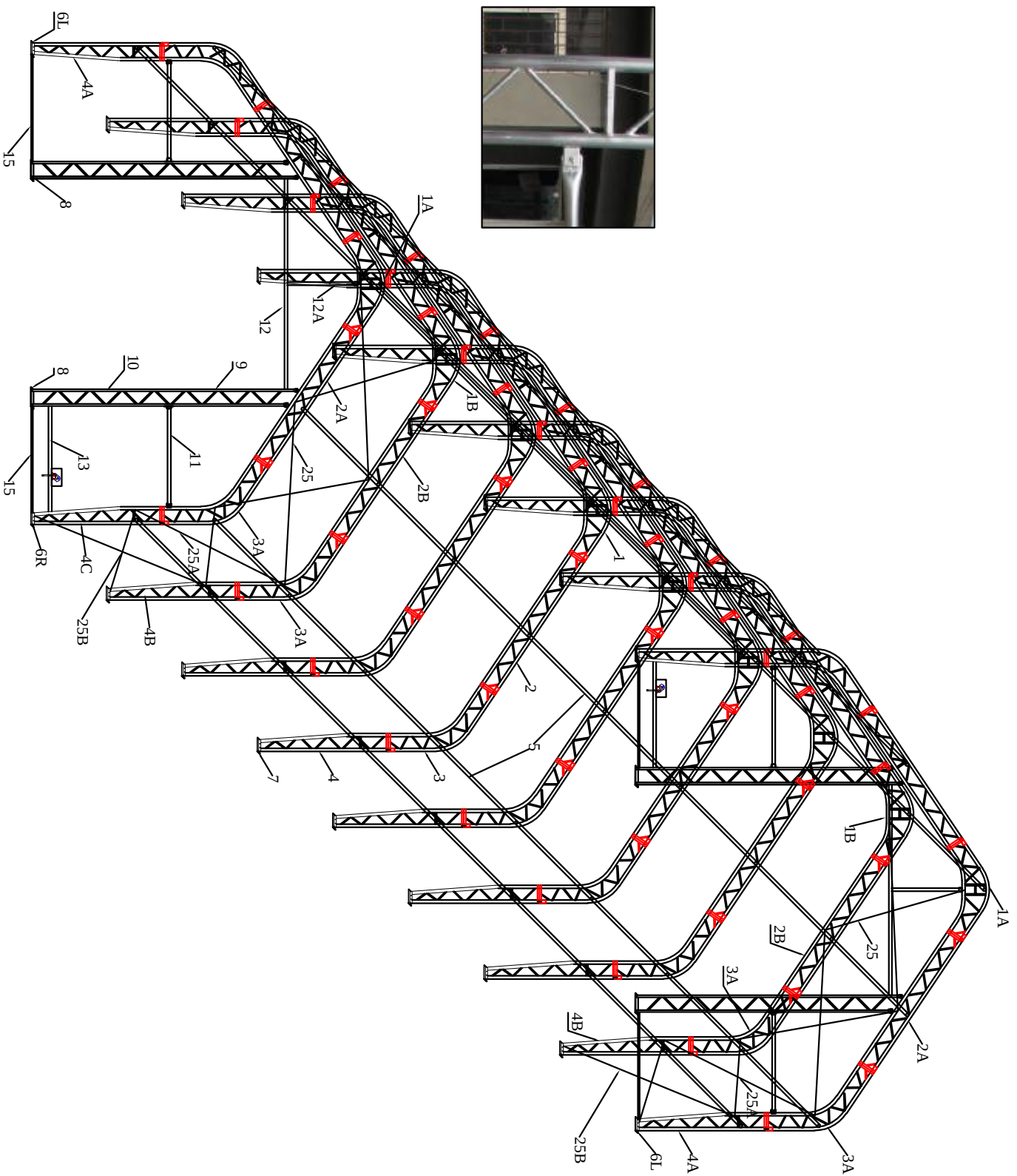
Figure 1 Sketch of Model 308022T Size: W9.15*L24.4*6.7M
