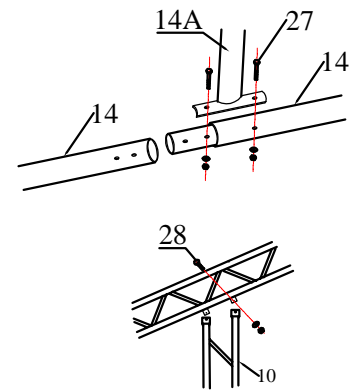
Figure 3 Front and Back Panel Arch
