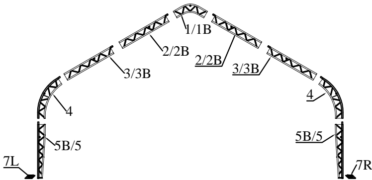
Figure 4 The middle arch
