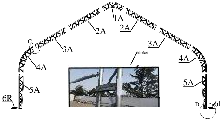
Figure 2 Front and Back Panel Arch
