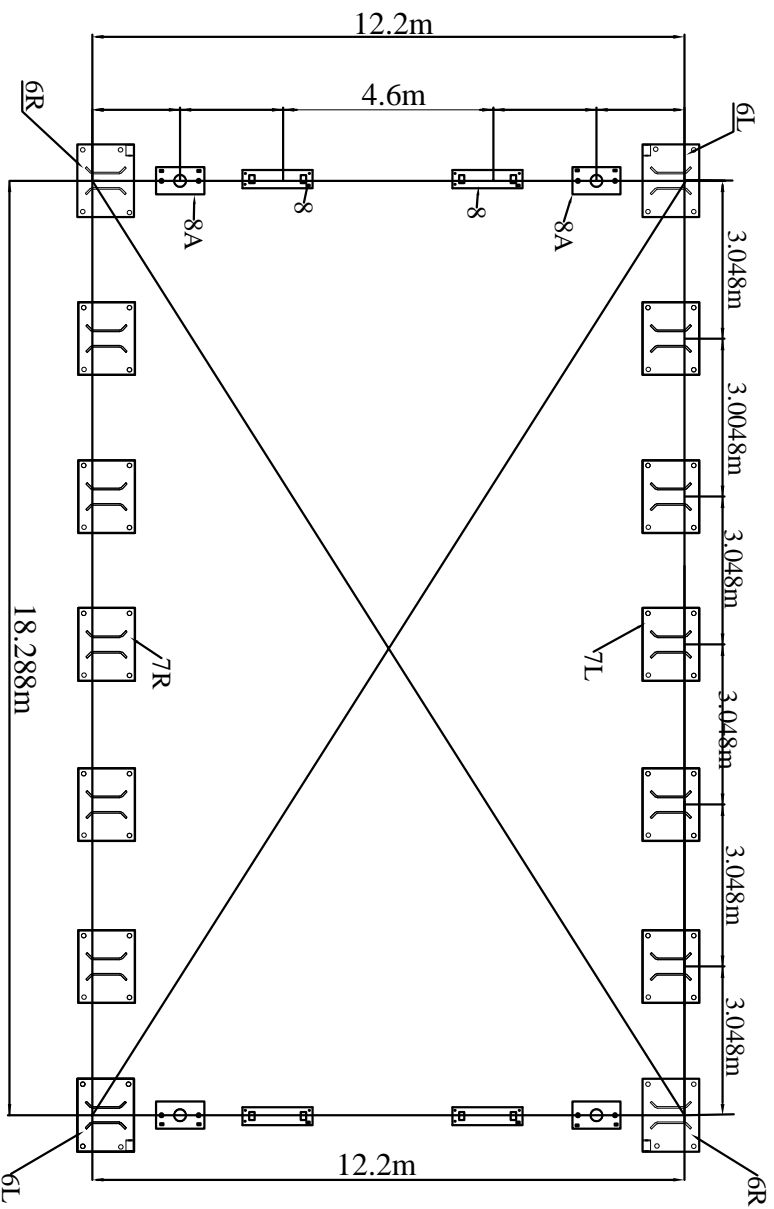
Figure 7 Position of Base Flanges
