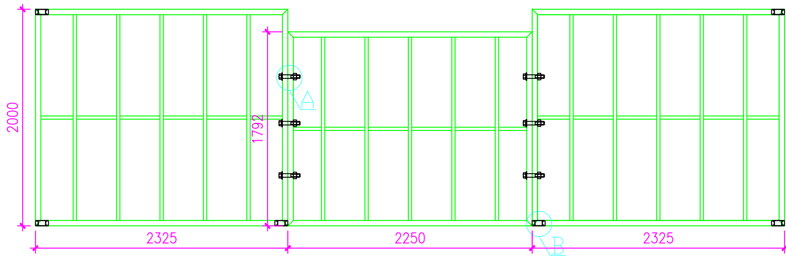
Bottom frame installation drawing
